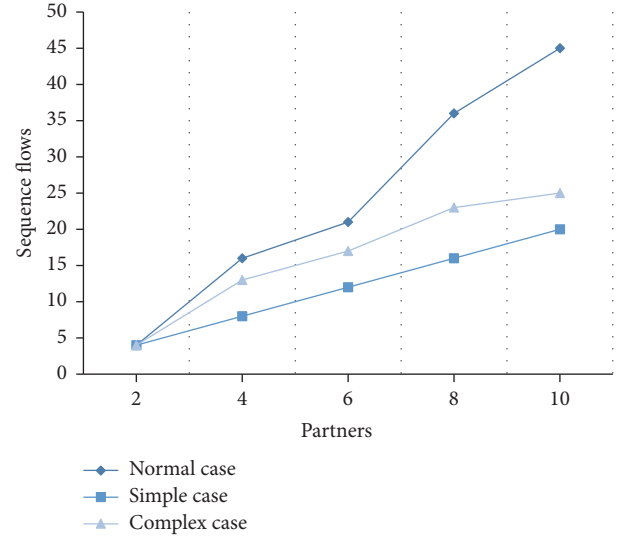
FIGURE 15: Number of sequences in different cases [9].
